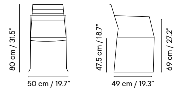
iSi 8002 Armchair
